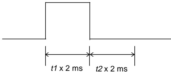
Figure 2.2.5 Drawer Kick-out Drive Signal
