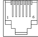
Figure 2.2.4 Drawer kick-out Connector
